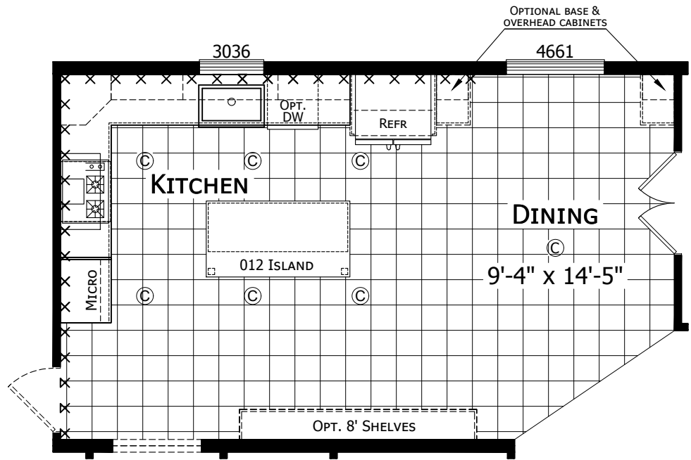
OPTIONAL ULTIMATE KITCHEN #2
